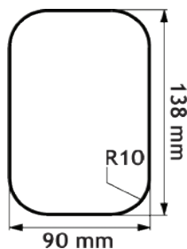
55018 Rubber Mounting Grommet
